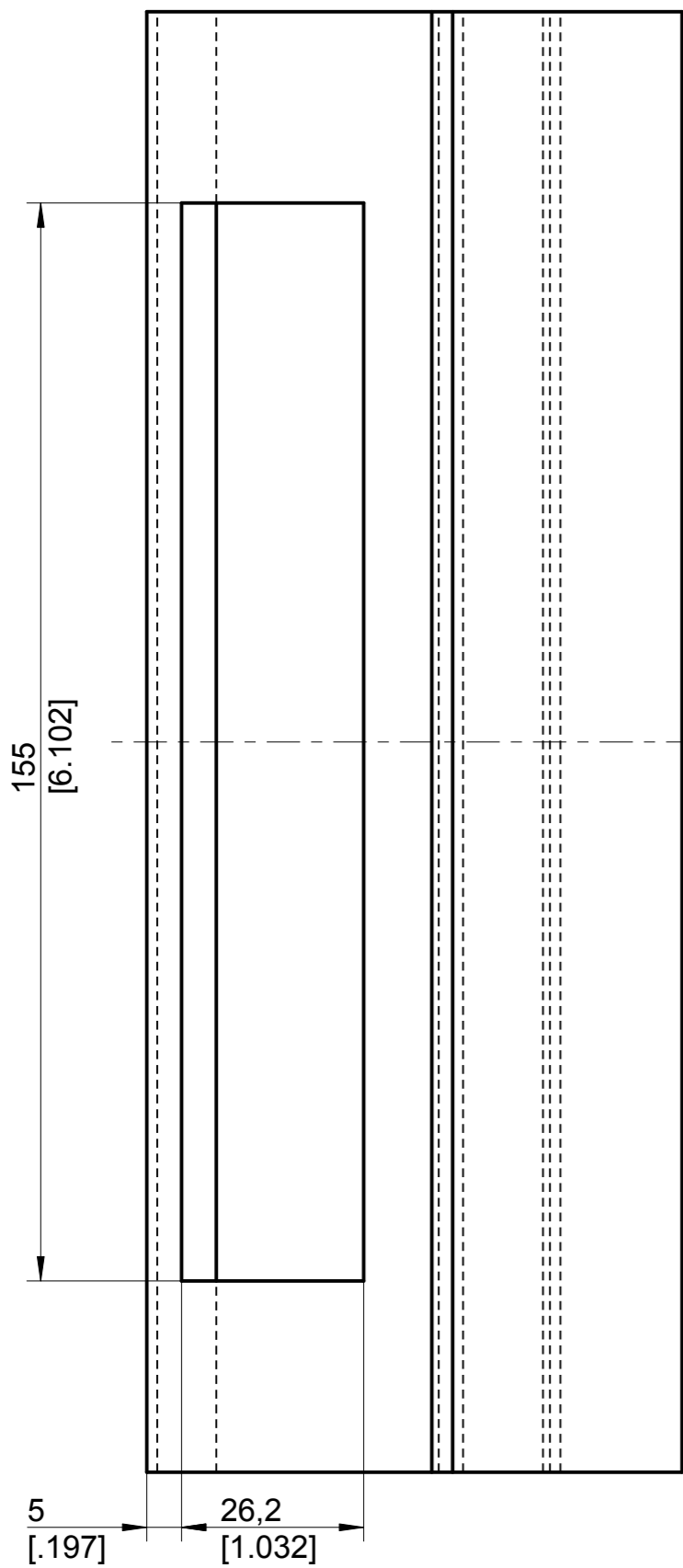
template steel frame
